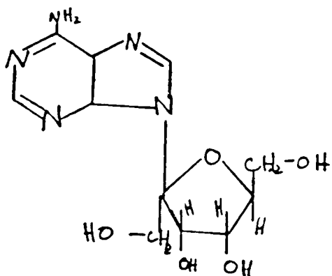
6-amino-9-psiicofuranosylpurine
