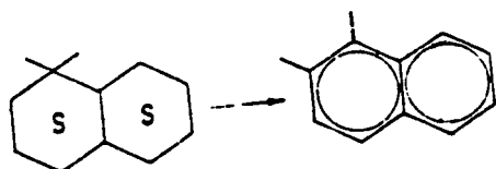
1,1-dimethyldecalin ; 1,2-dimethylnaphthalene
